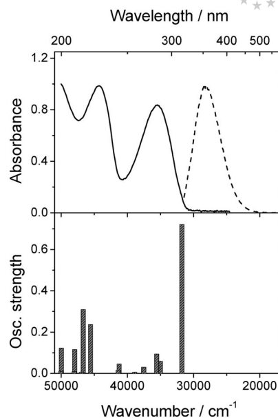
Figure 2. Absorption (solid line) and emission (dashed line) spectra of compound 7d in water (top). Calculated oscillator strengths and energies for the singlet-singlet electronic transitions below 50000\text{ cm}^{-1} (bottom).
