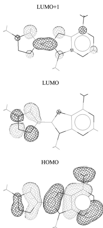
Figure 4. Frontier orbitals for the model compound 9-methyl-8-(1H-1,2,3-triazol-4-yl)adenine.
