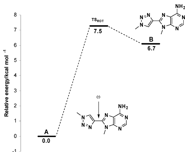
Figure 3. Potential energy surface and electrostatic potential of the model compound 9-methyl-8-(triazol-4-yl)adenine. Energies are calculated at the B3LYP/6-311G(d,p) level of theory.
