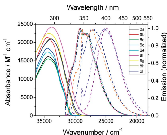
Figure 1. Absorption (solid line) and emission (dashed line) of nucleoside 6a–6i at room temperature in THF. The sharp peak at 347 nm for the weakly fluorescent derivatives is due to Raman scattering.
